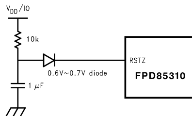
FIGURE 17. Delay Circuit for Stable RSTZ
