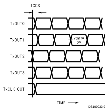
FIGURE 5. DS90CF383 (Transmitter) Channel-to-Channel Skew and Pulse Width
