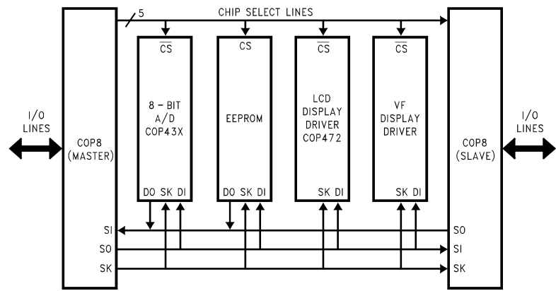
FIGURE 18. MICROWIRE/PLUS Application
