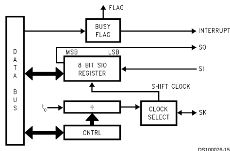
FIGURE 17. MICROWIRE/PLUS Block Diagram
