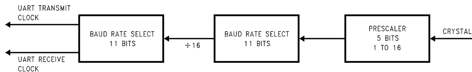
FIGURE 46. USART BAUD Clock Generation
