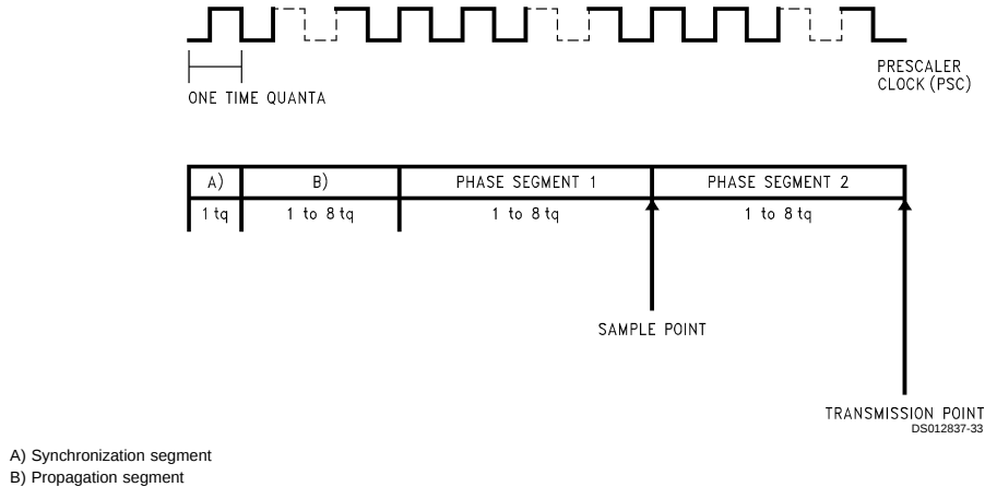
FIGURE 28. Bit Timing
