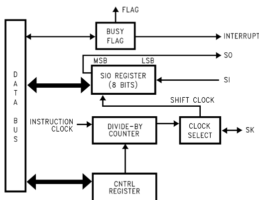
FIGURE 34. MICROWIRE/PLUS Block Diagram
