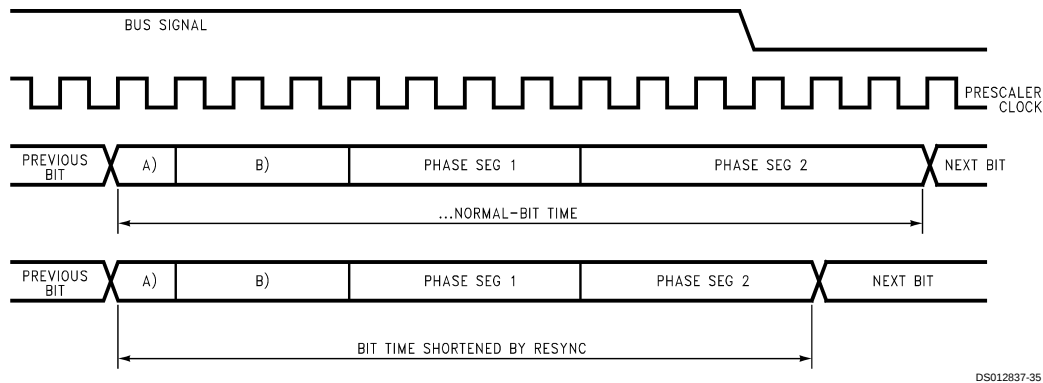
FIGURE 30. Resynchronization 2
