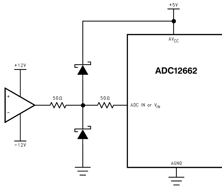
FIGURE 9. Input Protection
