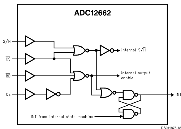
FIGURE 6. ADC Control Logic
