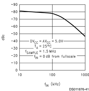
THD vs Input Frequency (ADC In)
