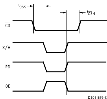
FIGURE 3. \overline{CS} Setup and Hold Timing for \overline{S/H} , \overline{RD} , and OE
