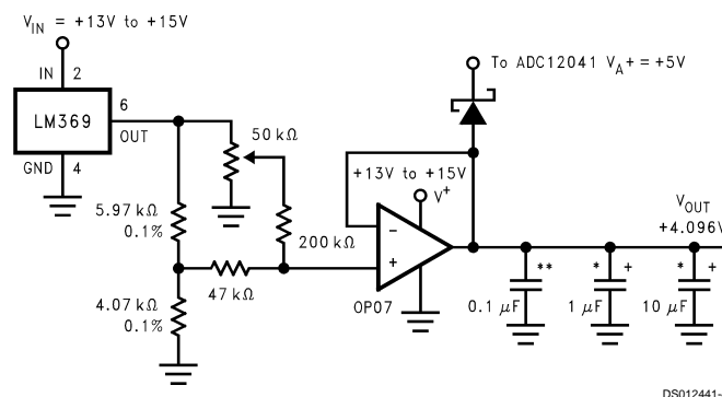
FIGURE 20. Low Drift Extremely Stable Reference Circuit
