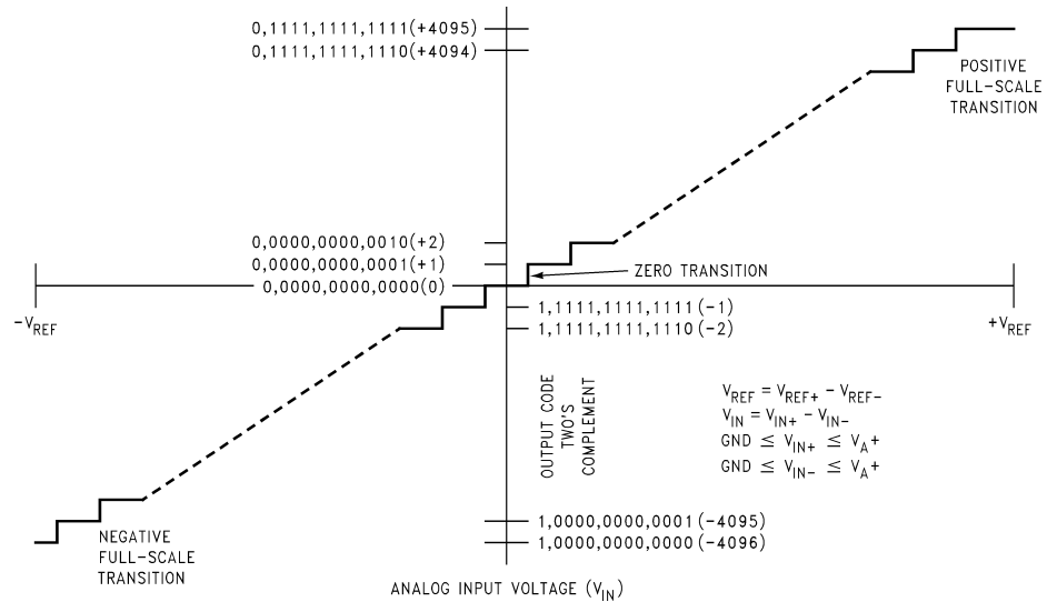
FIGURE 5. Transfer Characteristic
