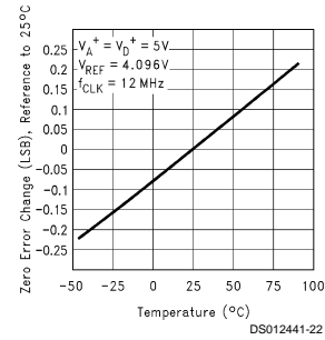
Zero Error Change vs Temperature
