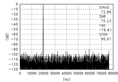
Half Scale Differential 20 kHz Sine Wave Input, f_S = 153.6\text{kHz}
