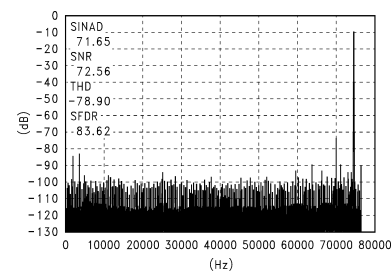
Half Scale Differential 75 kHz Sine Wave Input, f_S = 153.6\text{kHz}
