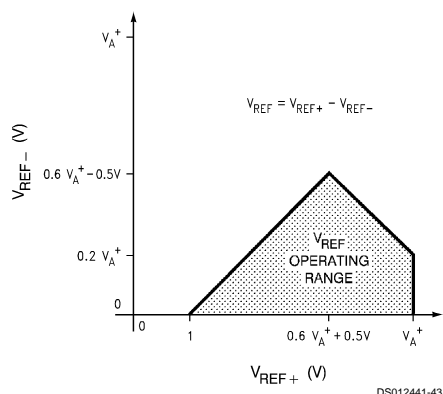
FIGURE 19. V_{REF} Operating Range
