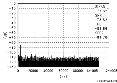
Full Scale Differential 1,099 Hz Sine Wave Input
