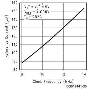
Reference Current vs Clock Frequency
