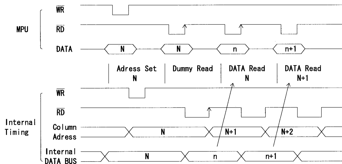
Fig.2 MPU Interface Timing
