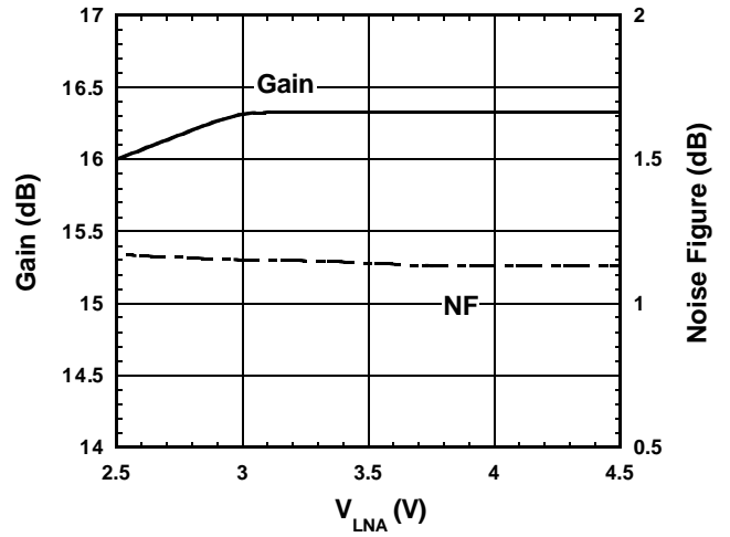
Gain, NF vs. V_{LNA} ( f=1900MHz )
