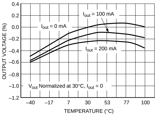
Figure 2. Normalized Output Voltage vs. Temperature
