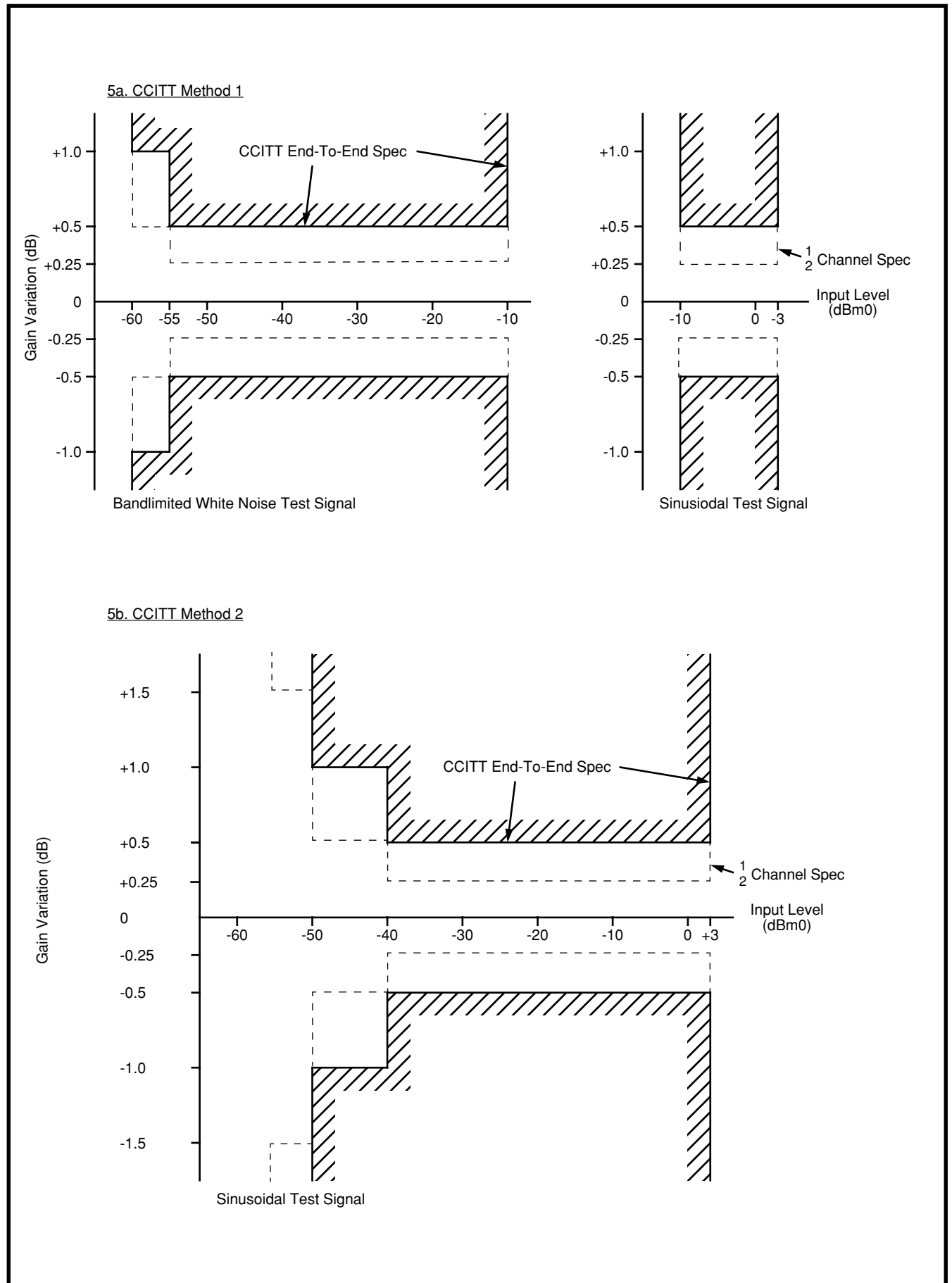
Figure 12 - Variation of Gain With Input Level
