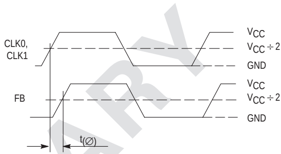
Figure 11. Propagation delay ( t_{\phi} , static phase offset) test reference
