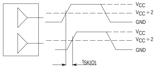
Figure 9. CLK0, CLK1 MPC9893 AC test reference for V_{CC} = 3.3V and V_{CC} = 2.5V
