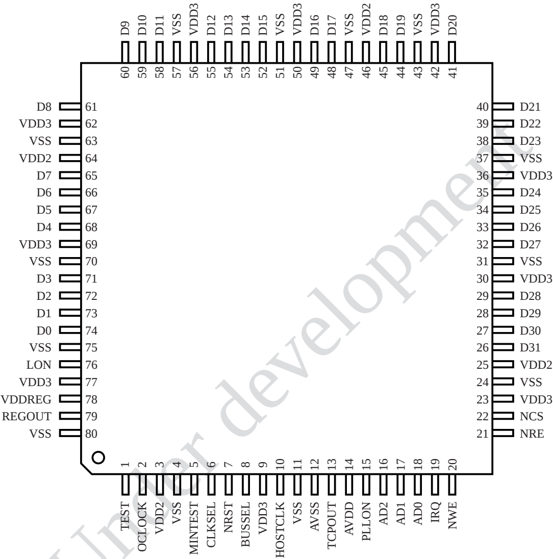
(TOP VIEW)
