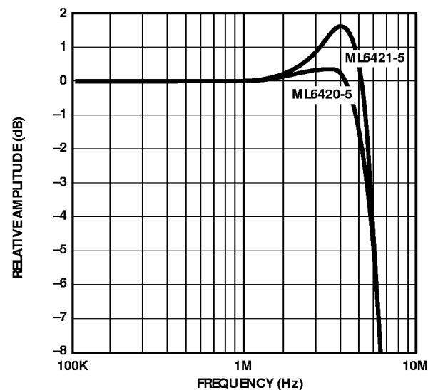
Figure 4. Pass-Band Amplitude vs Frequency ( f_c = 5.5\text{MHz} ).
