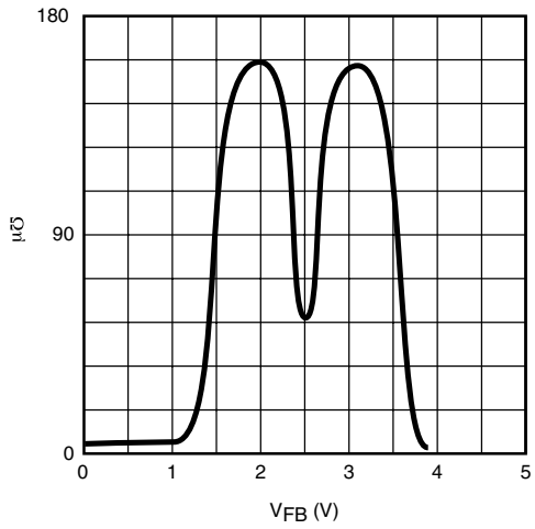
Figure 6. g_m of VOTA
