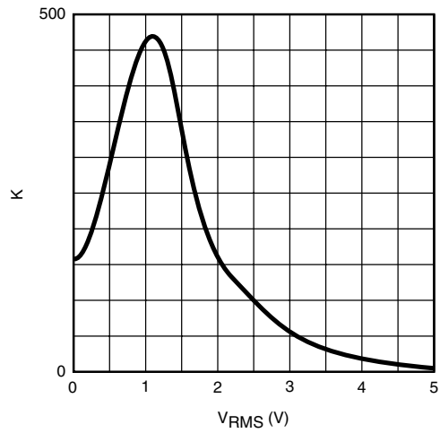
Figure 8. K of Multiplier
