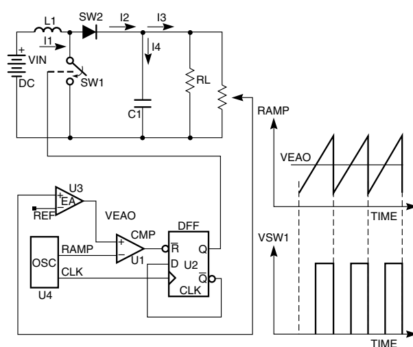
Figure 4. Leading/Trailing Edge Control Scheme
