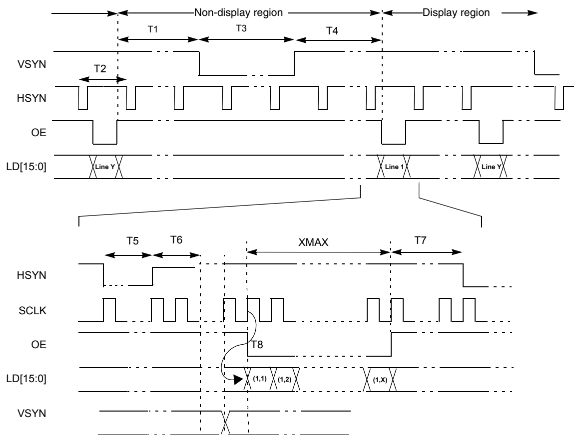
Figure 44. 4/8/16 Bit/Pixel TFT Color Mode Panel Timing Diagram
