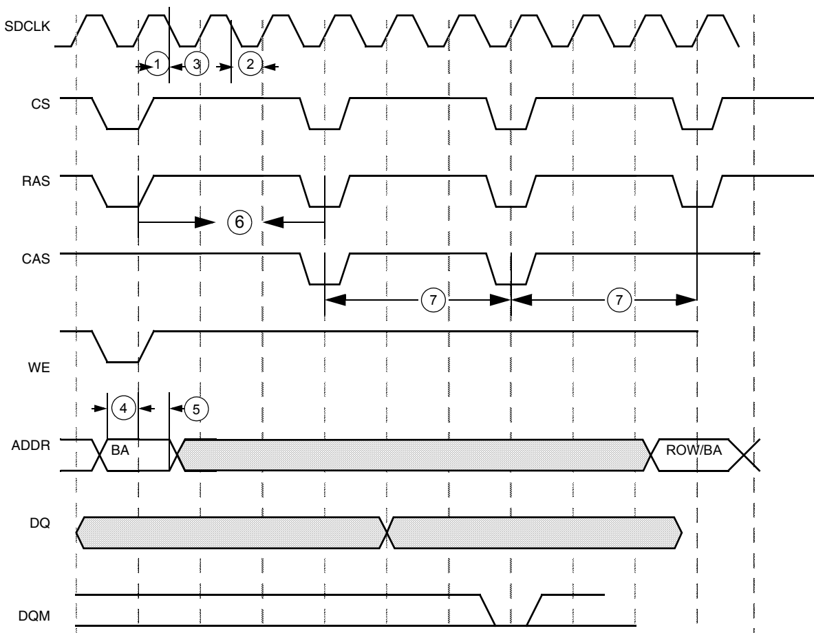
Figure 57. SDRAM Refresh Timing Diagram
