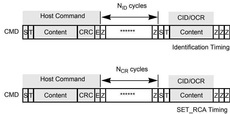
Figure 46. Timing Diagrams at Identification Mode
