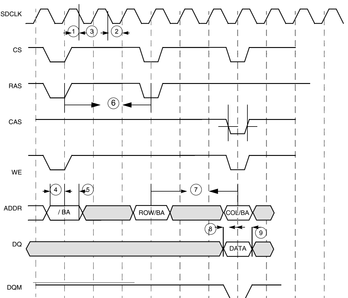
Figure 56. SDRAM/SyncFlash Write Cycle Timing Diagram
