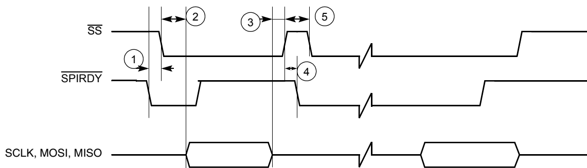
Figure 38. Master SPI Timing Diagram Using \overline{\text{SPI\_RDY}} Edge Trigger
