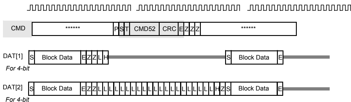
Figure 52. SDIO ReadWait Timing Diagram
