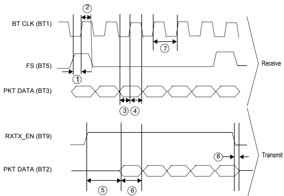
Figure 36. Motorola MC13180 Data Bus Timing Diagram
