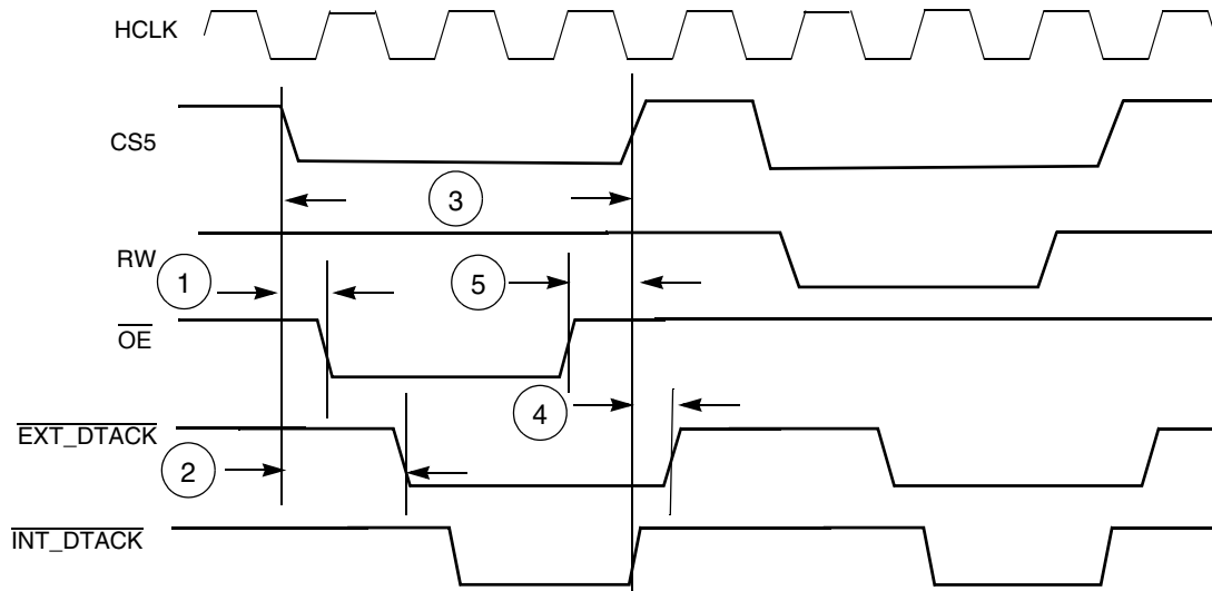
Figure 6. \overline{\text{DTACK}} Timing, WSC=111111, \overline{\text{DTACK\_sel}}=0
