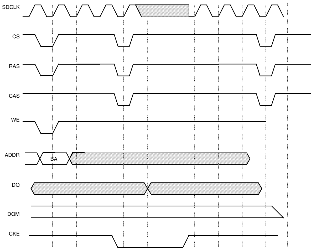
Figure 58. SDRAM Self-Refresh Cycle Timing Diagram
