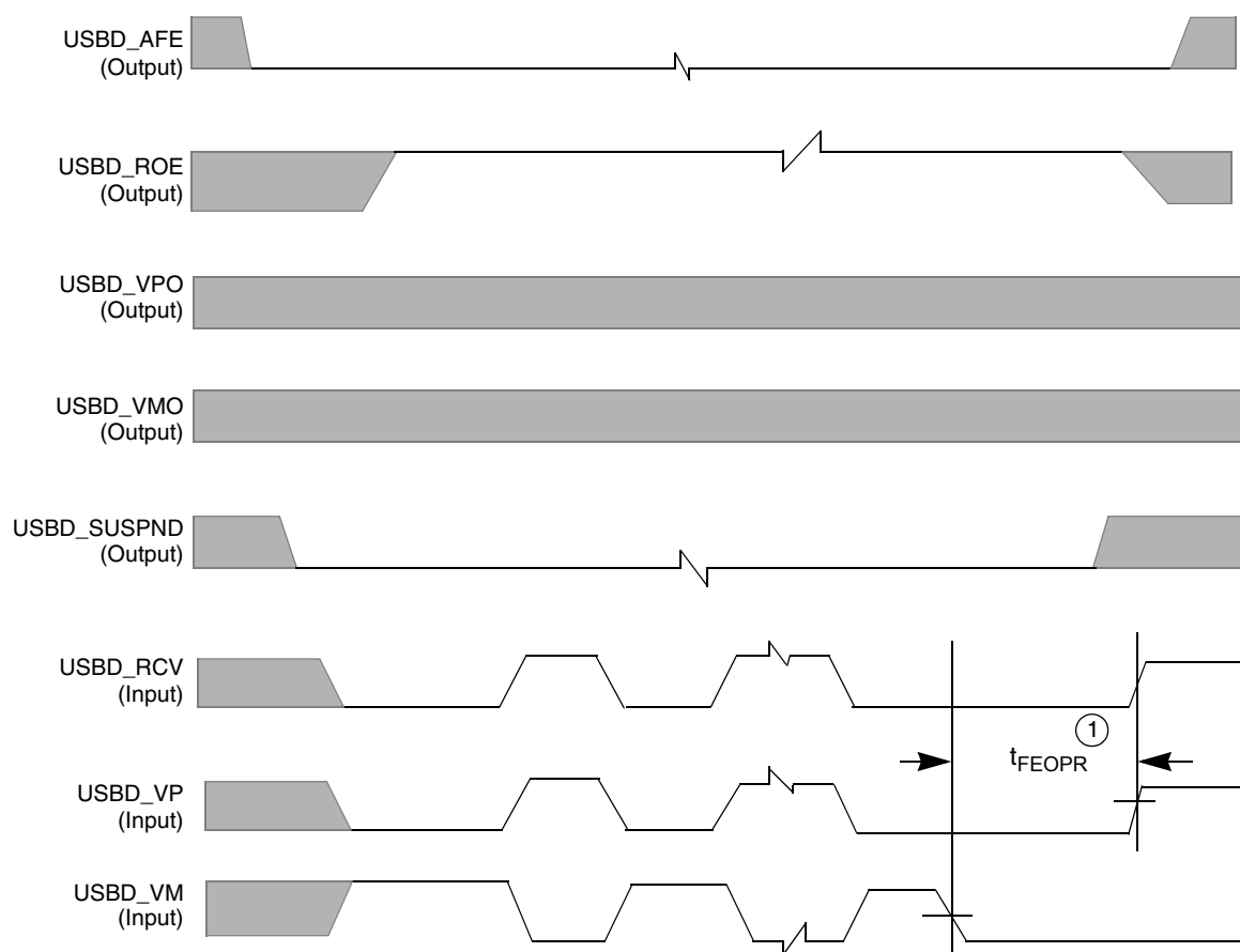
Figure 60. USB Device Timing Diagram for Data Transfer from USB Transceiver (RX)
