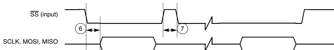
Figure 42. Slave SPI Timing Diagram FIFO Advanced by \overline{\text{SS}} Rising Edge
