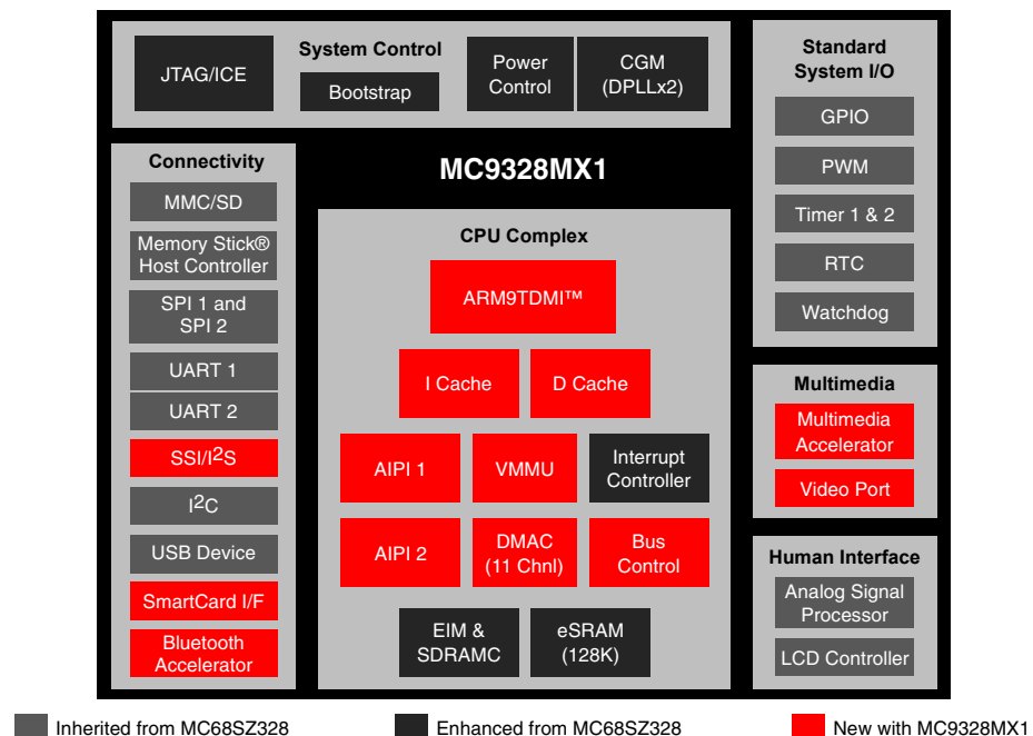
Figure 1. MC9328MX1 Functional Block Diagram
