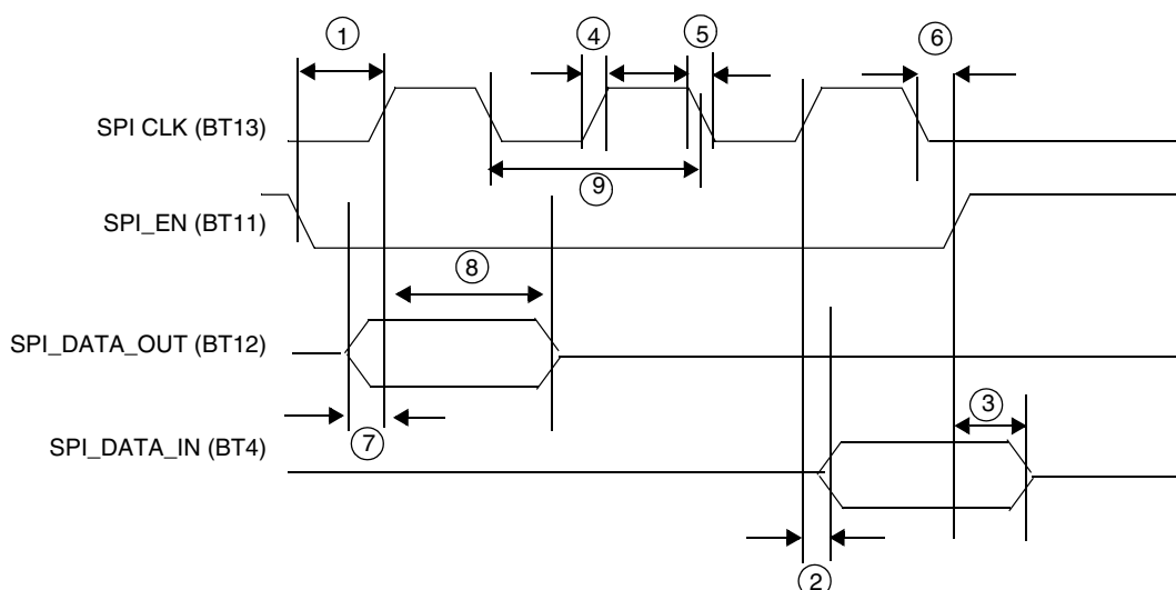
Figure 37. SPI Interface Timing Diagram Using Motorola MC13180
