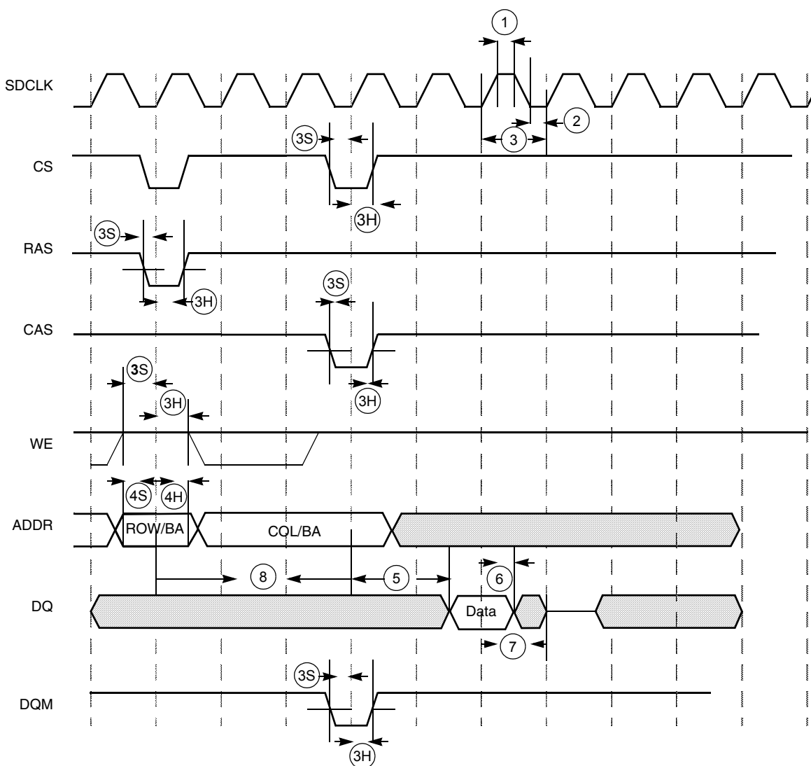
Figure 55. SDRAM/SyncFlash Read Cycle Timing Diagram
