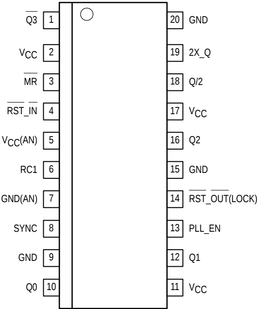
Pinout: 20-Lead Wide SOIC Package (Top View)
