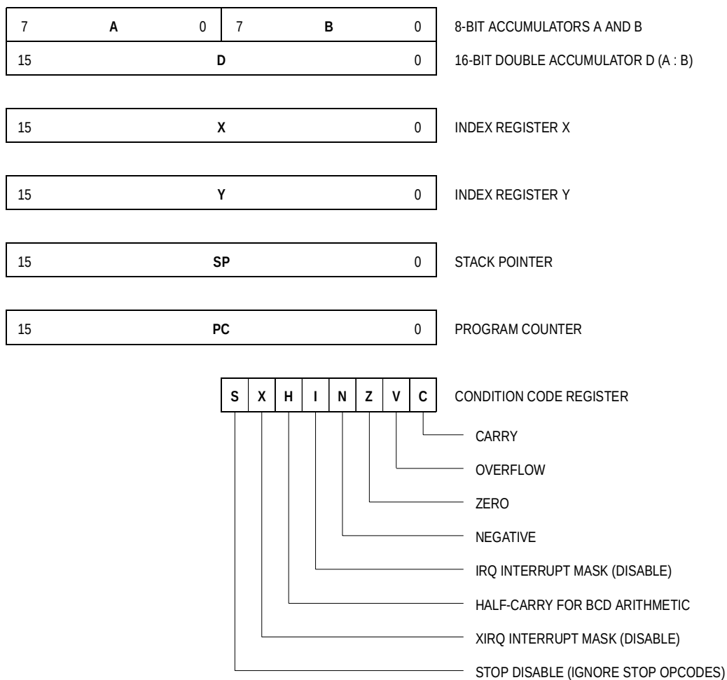
Figure 3-1. Programming Model
