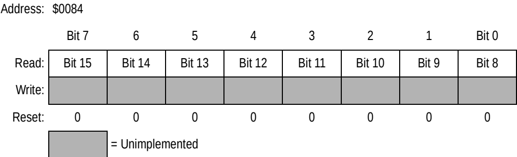
Figure 12-8. Timer Counter Register High (TCNTH)
