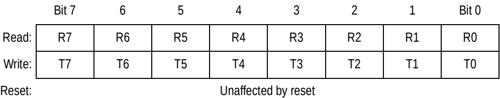
Figure 14-24. SCI Data Register Low (SC0DRL or SC1DRL)
