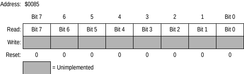
Figure 12-9. Timer Counter Register Low (TCNTL)
