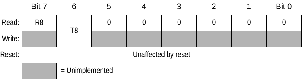
Figure 14-23. SCI Data Register High (SC0DRH or SC1DRH)
