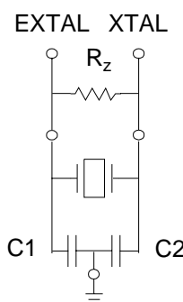
Figure 3-3 Connecting a Ceramic Resonator
