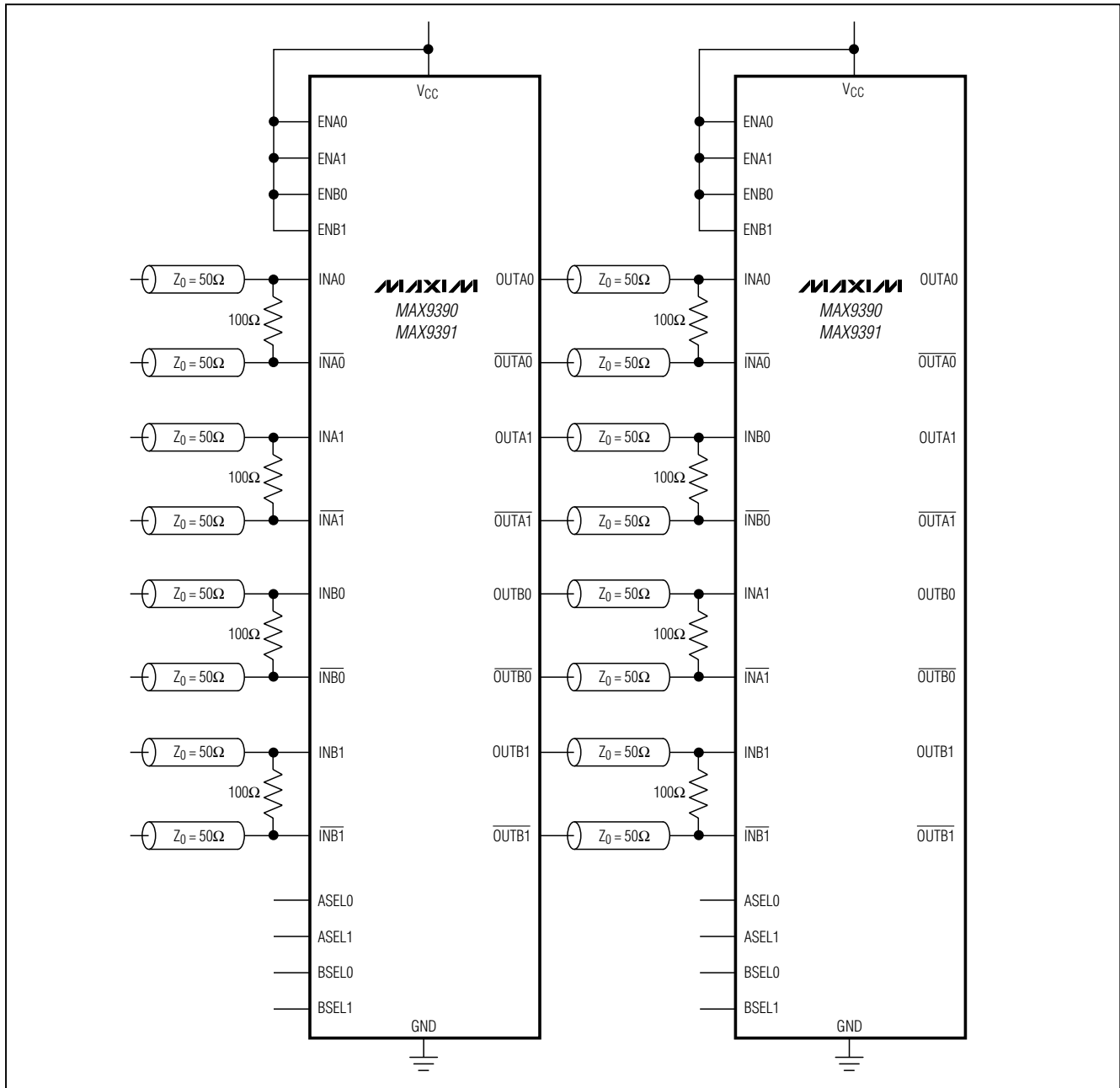
Figure 8. 4 Input x 4 Output Crosspoint Switch
