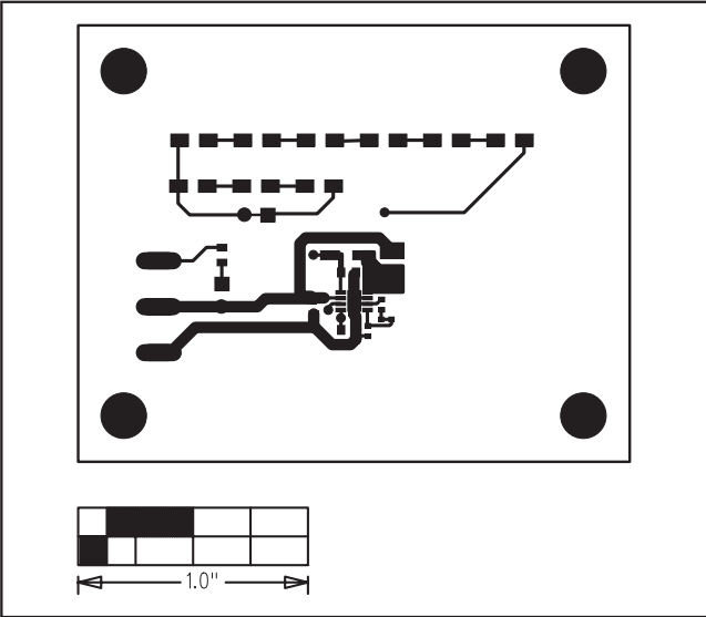
Figure 3. MAX8596Z EV Kit PC Board Layout—Component Side
