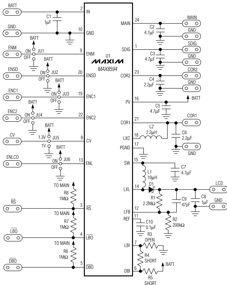
Figure 1. MAX8594 EV Kit Schematic
