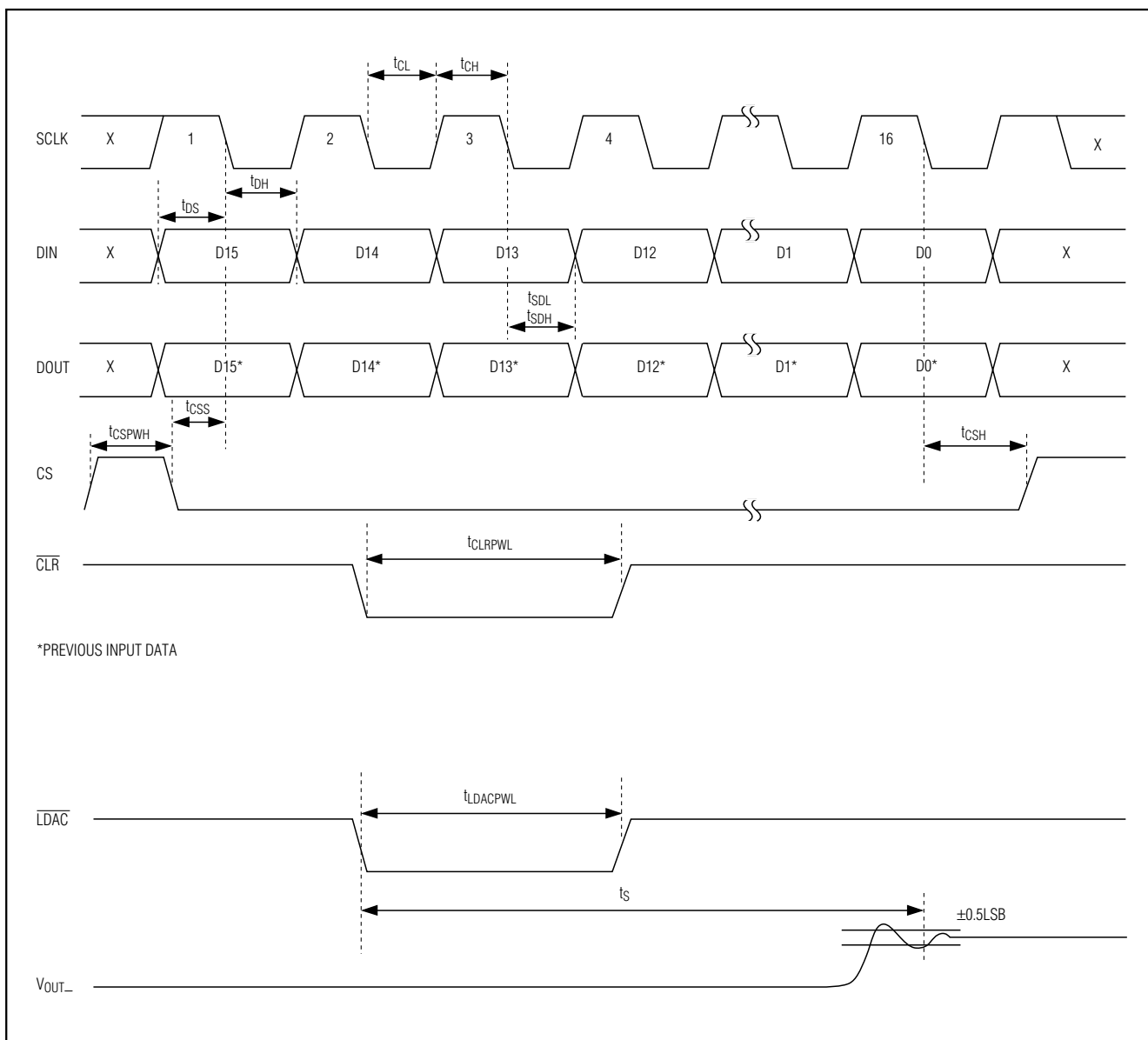
Figure 4. Timing Diagram
