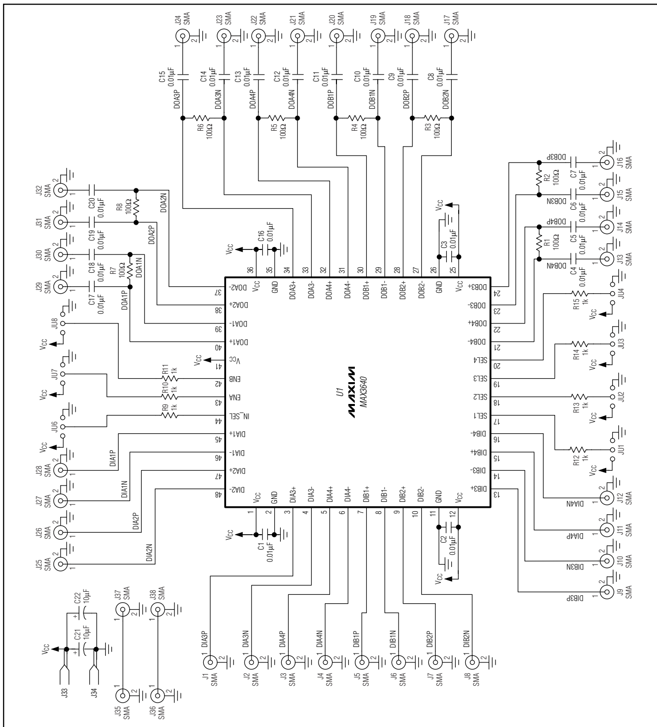
Figure 1. MAX3640 EV Kit Schematic
