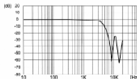
FIGURE 1. Characteristic of the low-pass filter at 8kHz sampling
