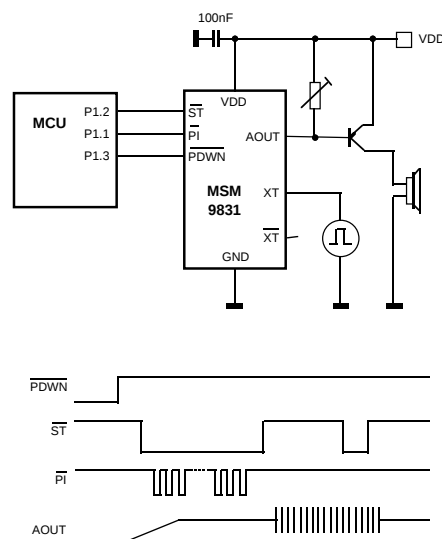
FIGURE 5. Principle playback and stop timing.
