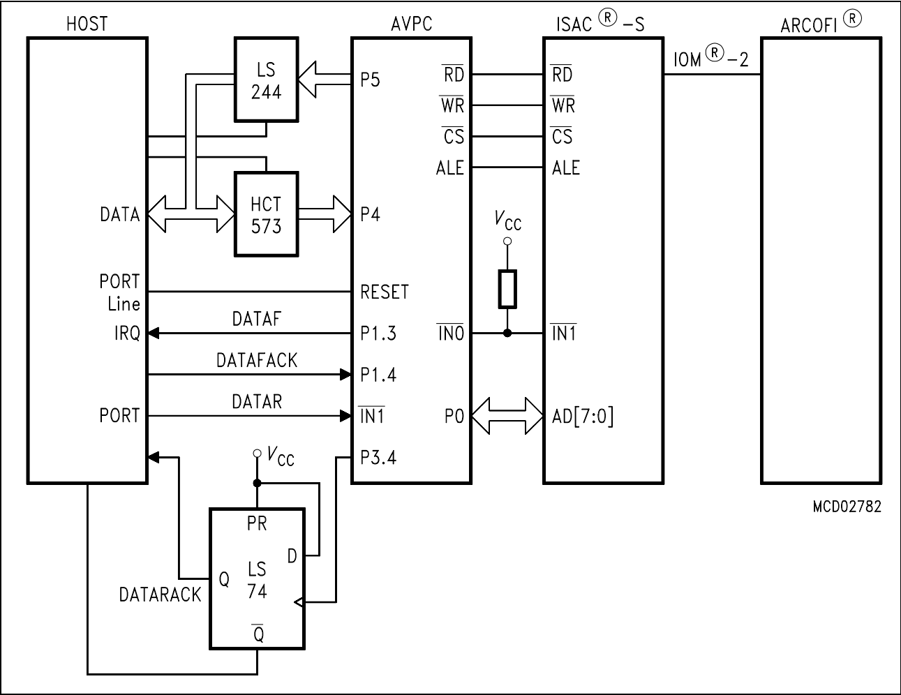
Figure 8 Hardware Block Diagram
