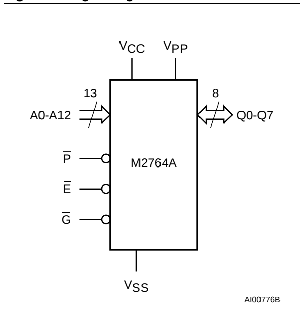
Figure 1. Logic Diagram
