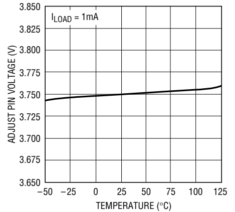
LT1529 Adjust Pin Voltage
