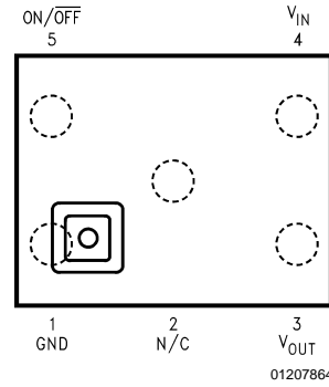
micro SMD, 5 Bump Package (BPA05)
