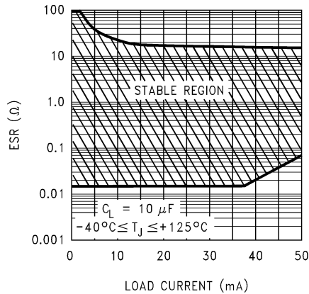
FIGURE 3. 10 \mu F ESR Range
