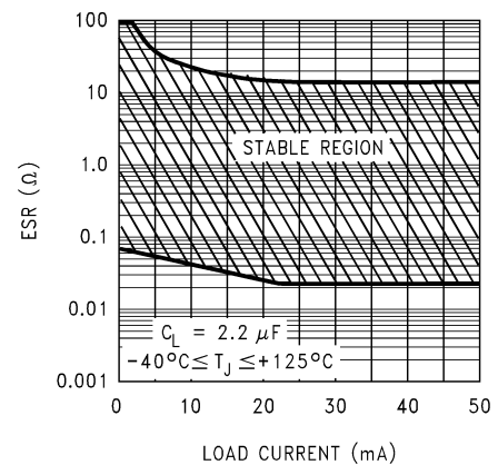
FIGURE 2. 2.2 \mu\text{F} ESR Range
