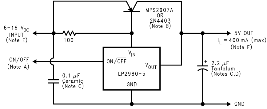
FIGURE 5. 5V/400mA Regulator
