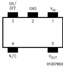
5-Lead Small Outline Package (M5)
