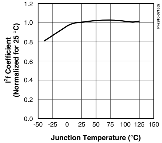
Figure 20. I²t Coefficient vs. Temperature.
