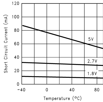
Short Circuit Current vs. Temperature (sinking)
