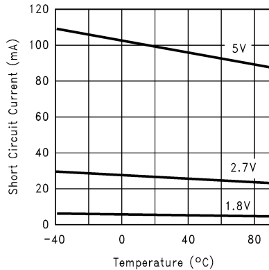
Short Circuit Current vs. Temperature (sourcing)
