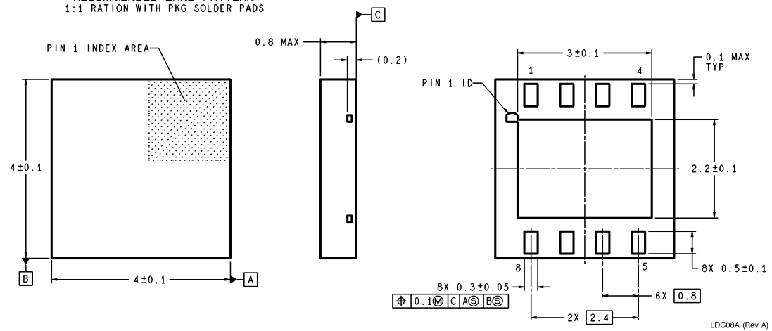
8-Pin LLP NSC Package Number LDC08A
