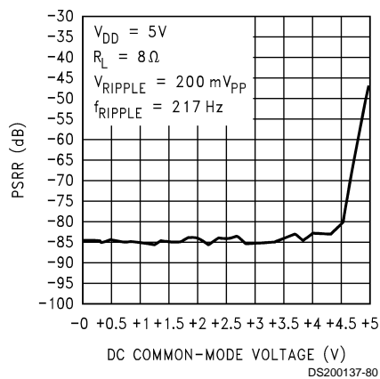
PSRR vs DC Common-Mode Voltage
