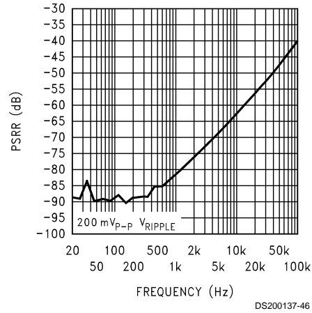
Power Supply Rejection Ratio (PSRR) V_{DD} = 5V Input Floating
