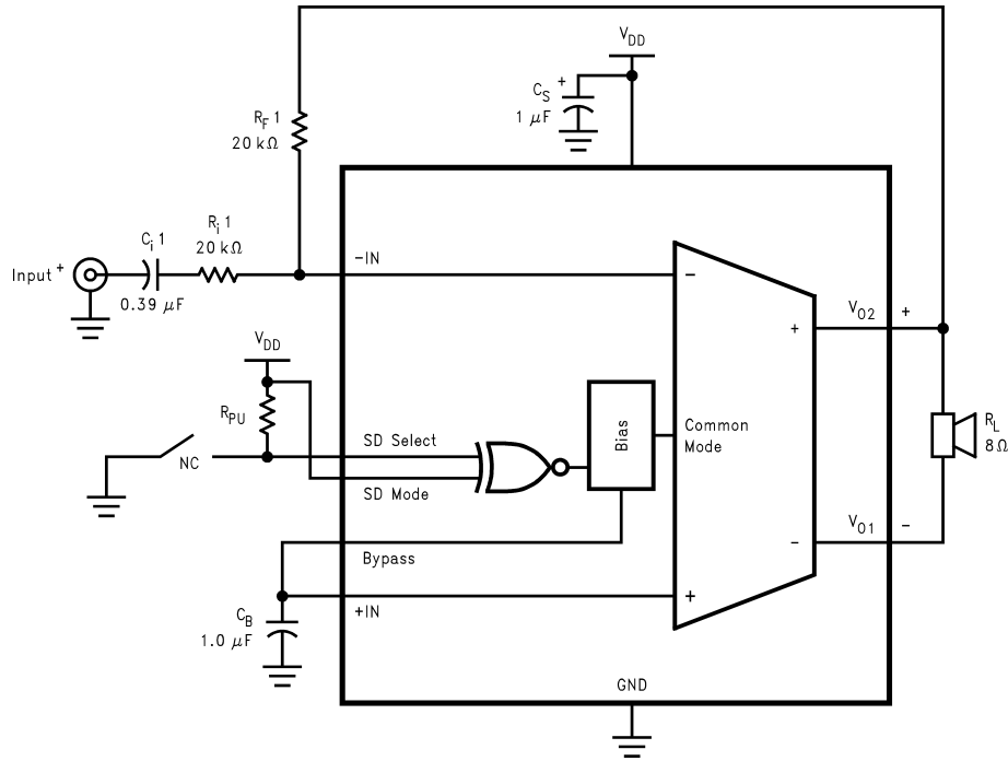
FIGURE 4. Single-Ended Input, "Shutdown-High" Configuration
