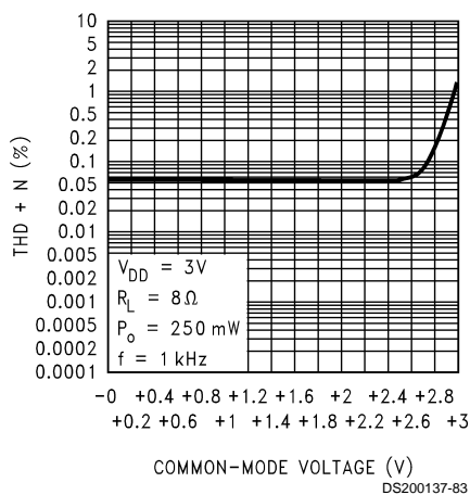
THD vs Common-Mode Voltage
