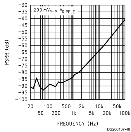
Power Supply Rejection Ratio (PSRR) V_{DD} = 3V Input Floating
