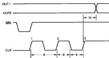
Figure 6. CLOCK to Output When Writing to PW Latch.
