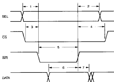
Figure 3. Write Operation Timing Diagram
