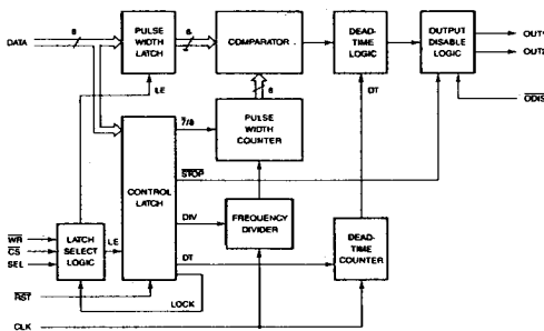
FUNCTIONAL IXDP610 BLOCK DIAGRAM
