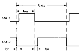
Figure 1. PWM Cycle Time and Dead-Time Definition
