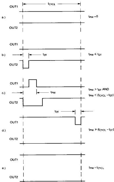
Figure 9. Effect of Nonzero Dead-time on PWM Waveform
