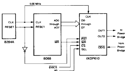
Figure 8. 8088 to IXDP610 Interface
