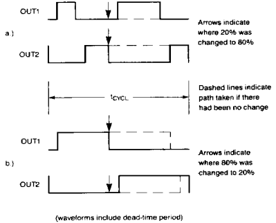
Figure 10. Effect of Changing the Duty Cycle during a PWM Cycle
