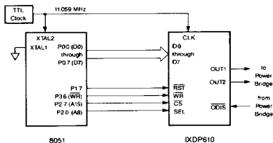
Figure 7. 8051 to IXDP610 Interface
