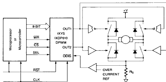
Figure 2. IXDP610 to DC Servo Motor Full Bridge Block Diagram
