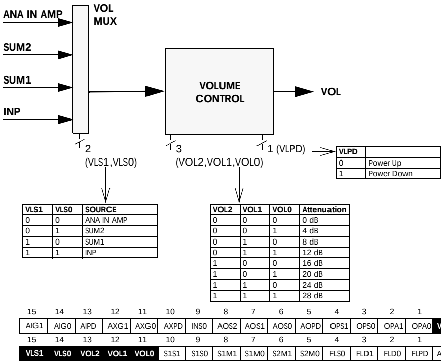
Figure 9: Volume Control
