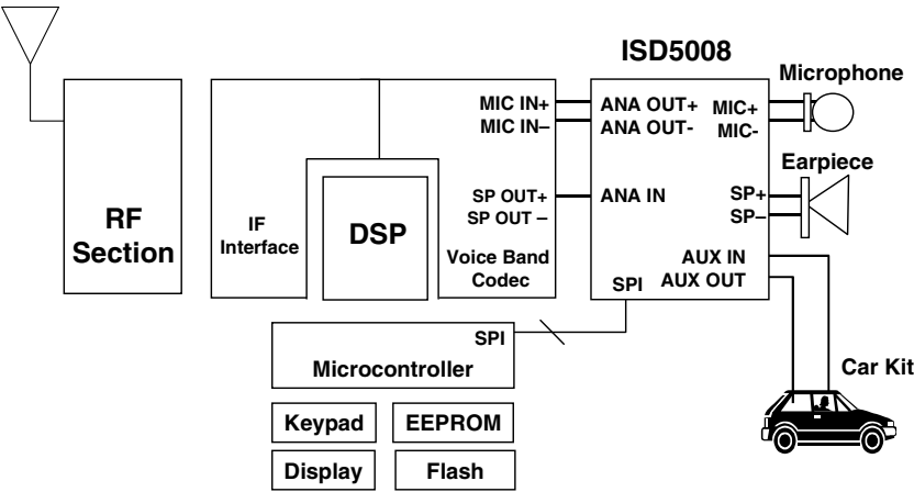
Figure 15: Typical Digital Cellular Phone Integration
