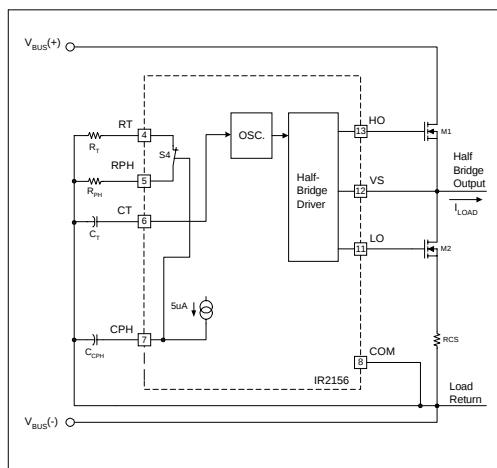
Figure 3, Preheat circuitry.
