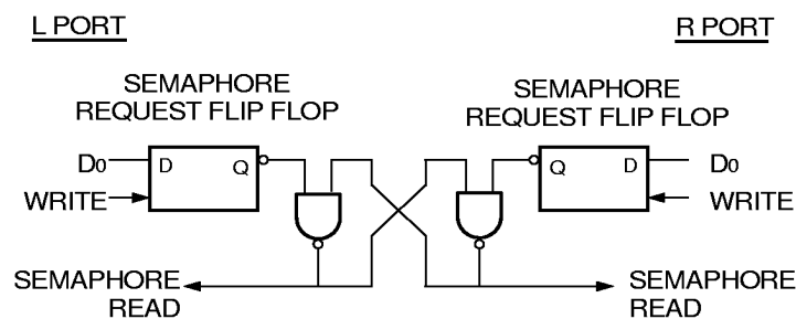
Figure 4. IDT7005 Semaphore Logic
