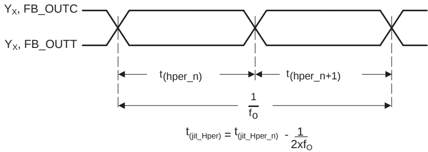
Figure 7. Half-Period Jitter
