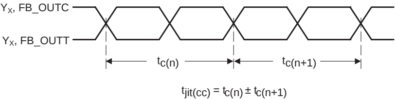
Figure 3. Cycle-to-Cycle Jitter
