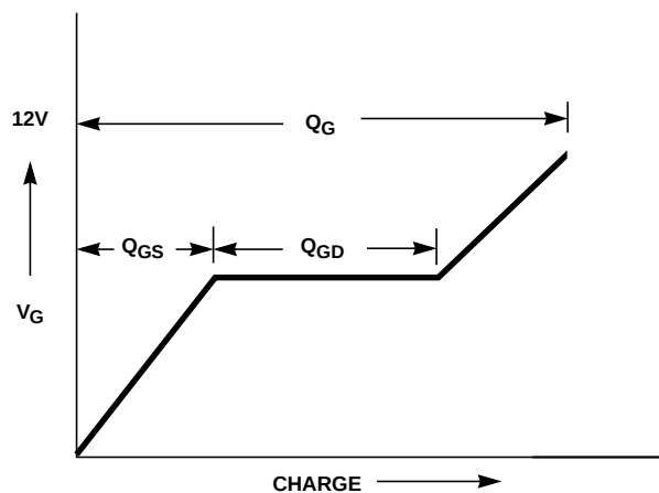
FIGURE 6. BASIC GATE CHARGE WAVEFORM
