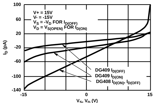
DRAIN LEAKAGE CURRENT vs SOURCE/DRAIN VOLTAGE
