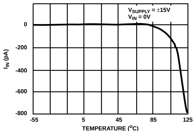
LOGIC INPUT CURRENT vs TEMPERATURE
