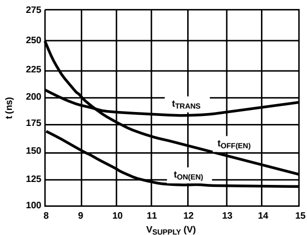
SWITCHING TIME vs V_{IN} (SINGLE SUPPLY)
