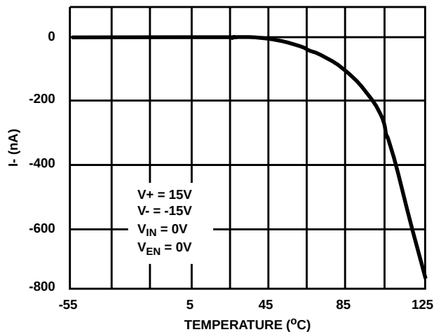
NEGATIVE SUPPLY CURRENT vs TEMPERATURE
