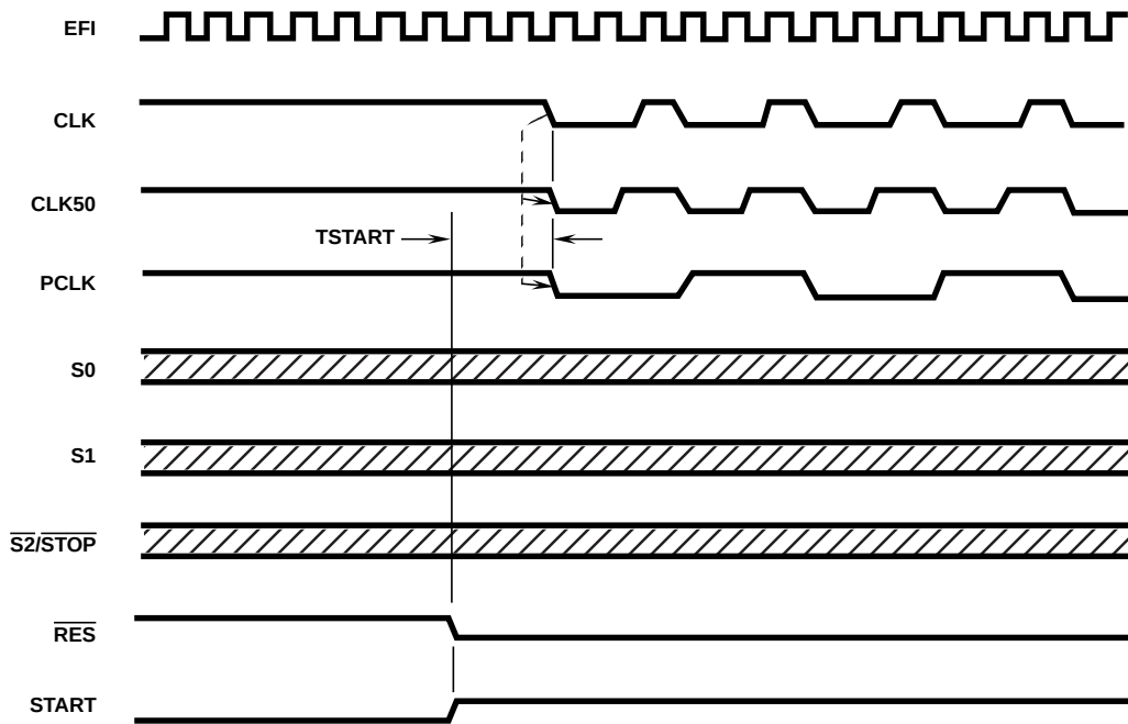
FIGURE 5. CLOCK START ( \overline{F/C} HIGH)
