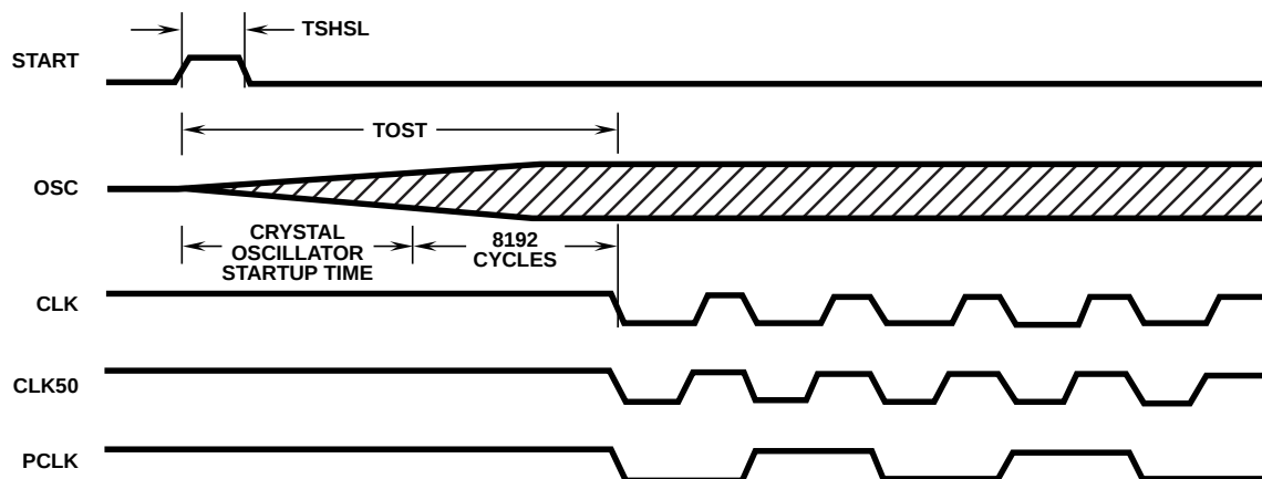
FIGURE 6. CLOCK START ( \overline{F/C} LOW)
