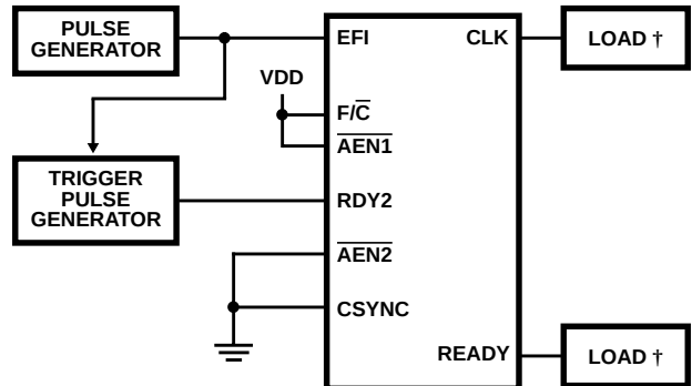
FIGURE 15. READY TO CLOCK (USING EFI)
