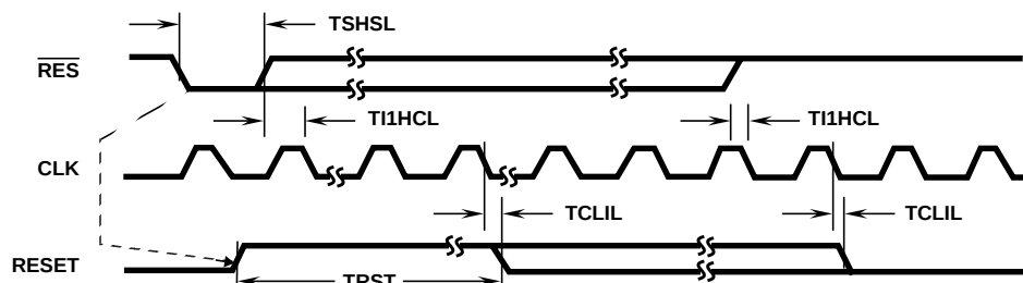
FIGURE 7. RESET TIMING (CLK RUNNING WITH \overline{F/C} LOW - OSC MODE; CLK RUNNING - OR STOPPED WITH \overline{F/C} HIGH EFI MODE)
