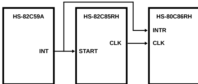
FIGURE 16. START CONTROL USING HS-82C59ARH INTERRUPT CONTROLLER
