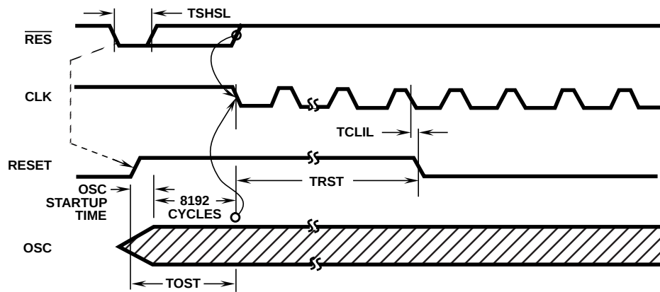
FIGURE 8. RESET TIMING OSCILLATOR STOPPED (F/C LOW)
