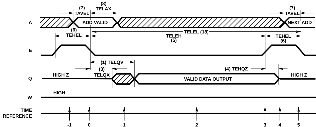
FIGURE 11. READ CYCLE
