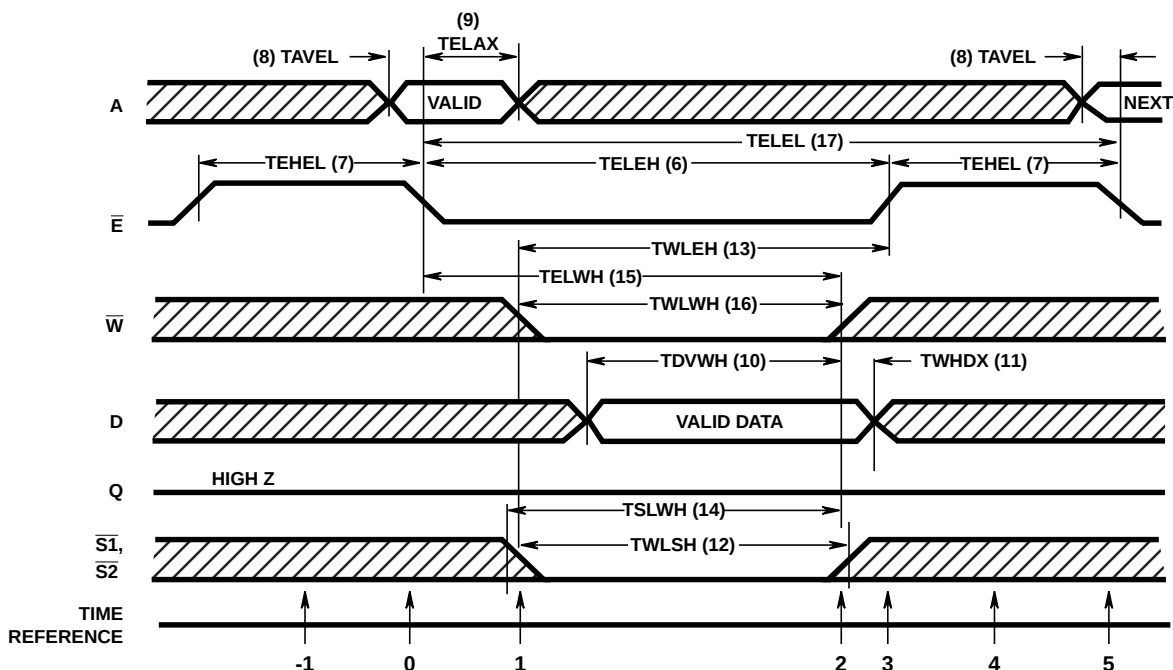
FIGURE 2. WRITE CYCLE
