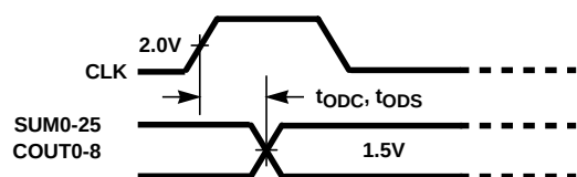
FIGURE 10. SUM0-25, COUT0-8, OUTPUT DELAYS
