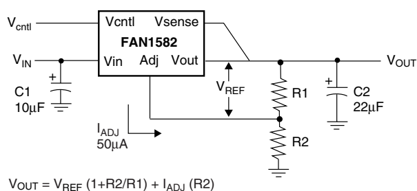
Figure 2. Basic Regulator Circuit
