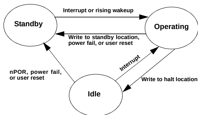
Figure 3. State Diagram
