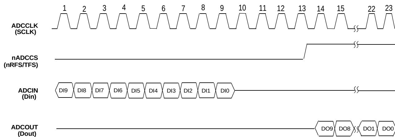
Figure 17. SSI Interface for AD7811/2
