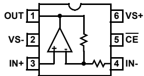
EL5108 (6-PIN SOT-23) TOP VIEW
