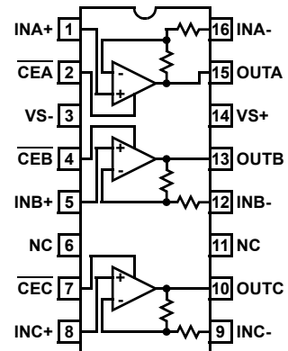
EL5308 (16-PIN SO, QSOP) TOP VIEW
