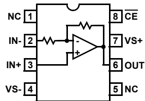
EL5108 (8-PIN SO) TOP VIEW
