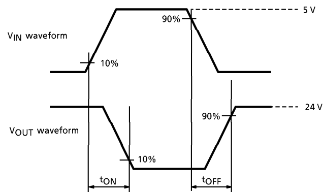
Measured waveforms
