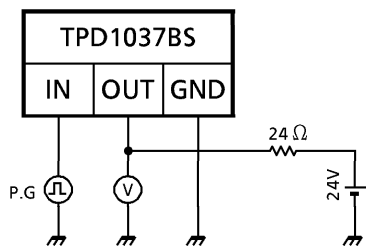
Test circuit
