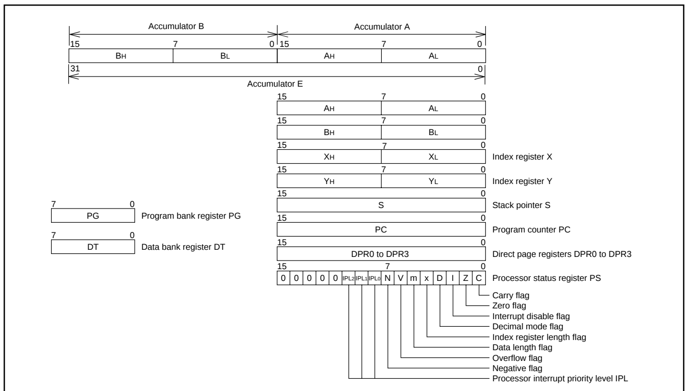
Fig. 9 Register structure
