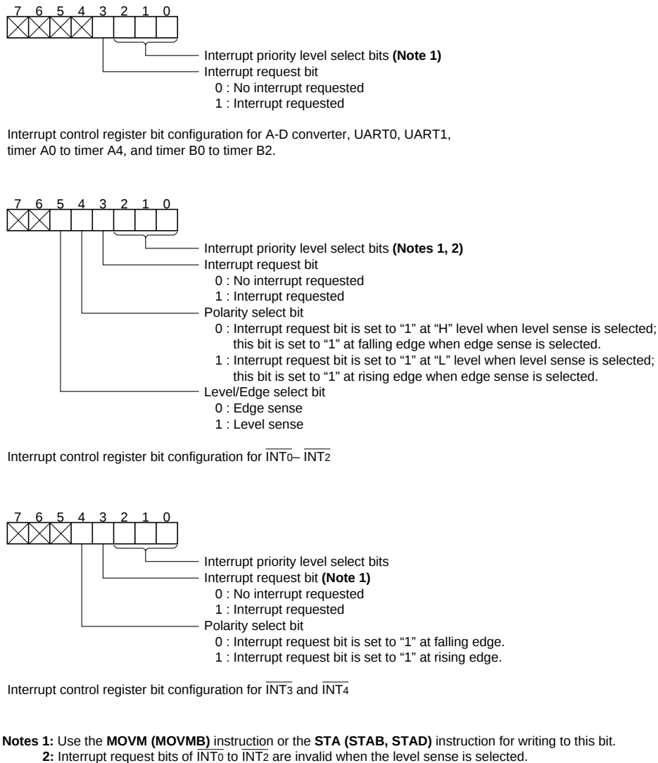
Fig. 35 Bit configuration of interrupt control register
