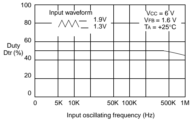
7. Duty - input oscillating frequency characteristic
