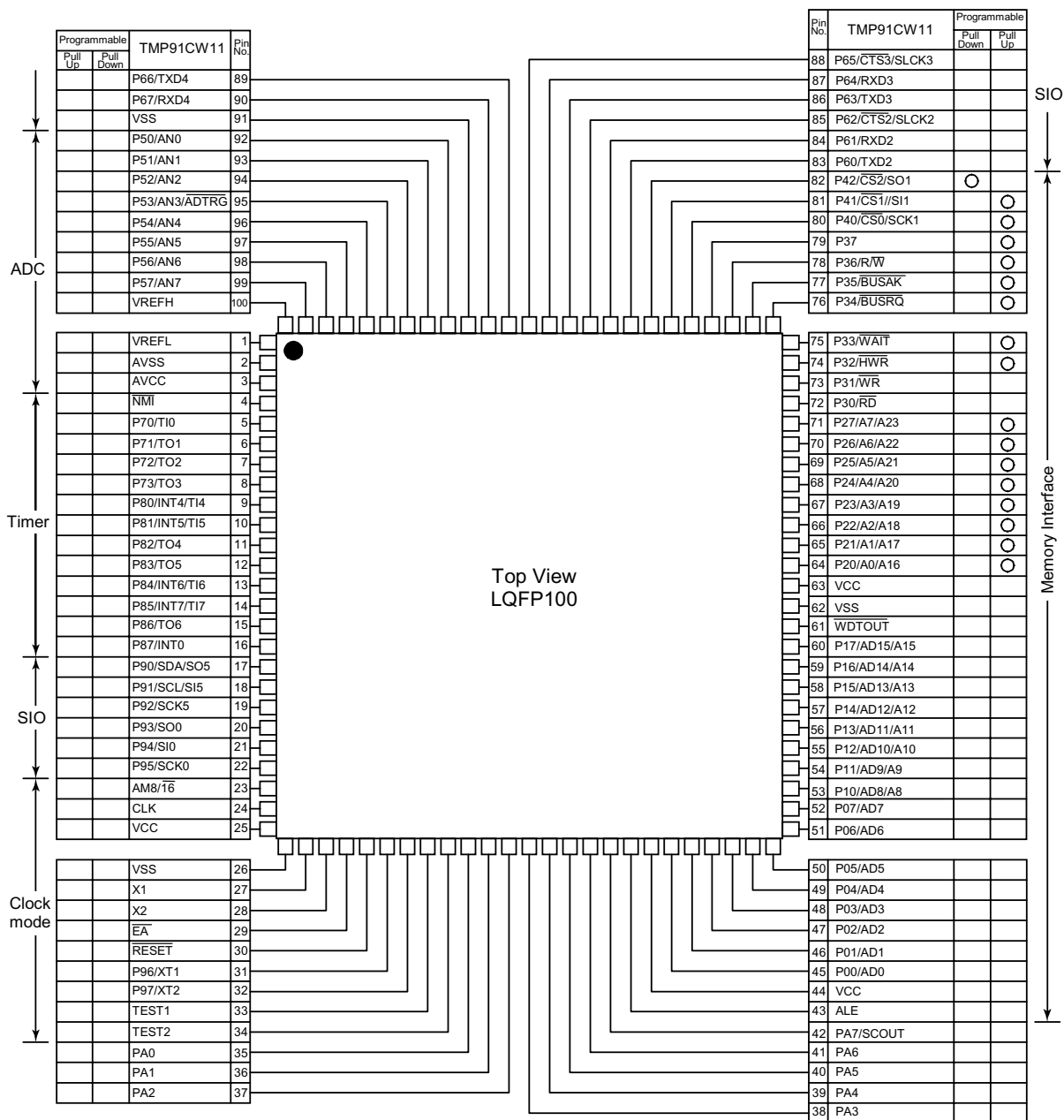
Figure 2.1.1 Pin assignment
